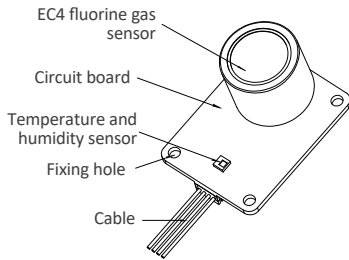
Product Schematic
